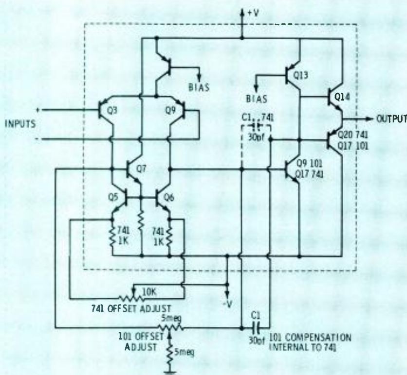
Fig. 4 Simplified schematic showing basic structure and differences in 741 and 101 type op-amps.
