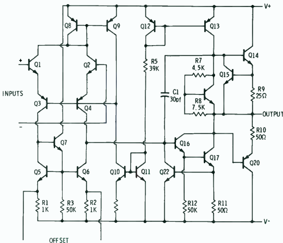
Fig. 3 Schematic of 741 type operational amplifier.
