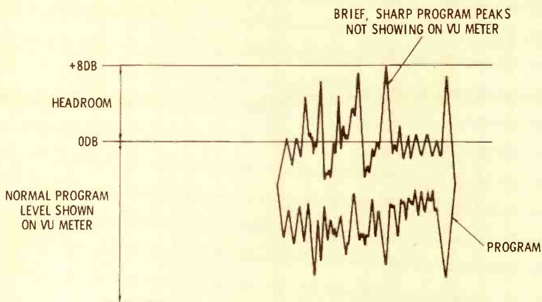
Fig. 5 System levels should allow "head-room" for signal peaks to clear without being clipped with resulting distortion. These brief, sharp peaks will not show up on the VU meter. System should be able to handle at least 8 dB above normal program levels without distortion.
