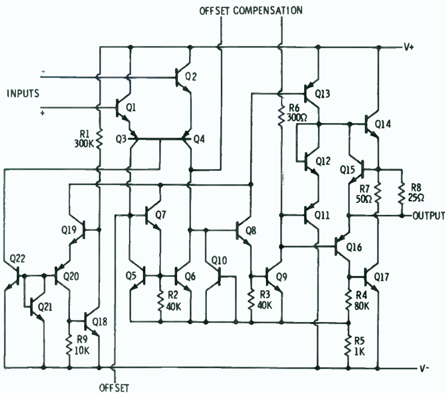
Fig. 2 Schematic of 101 type operational amplifier.
