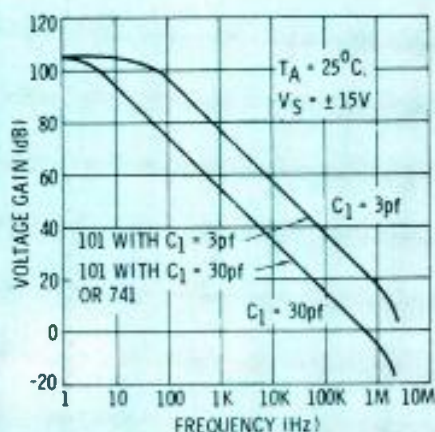
Fig. 5 Open loop response of 741 and 101 amplifiers. Note extra bandwidth available with 101 (3 pf curve).
